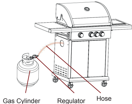
Illustration for the connection of Gas Cylinder, Regulator and Hose
